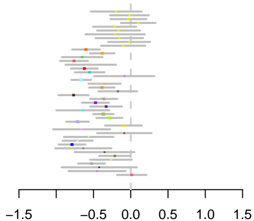
ENSG00000267508.1 SNP 2 in joint analysis
