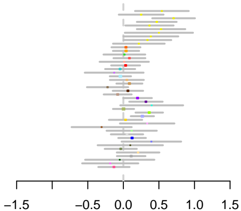
ENSG00000267508.1 SNP 1 in joint analysis
